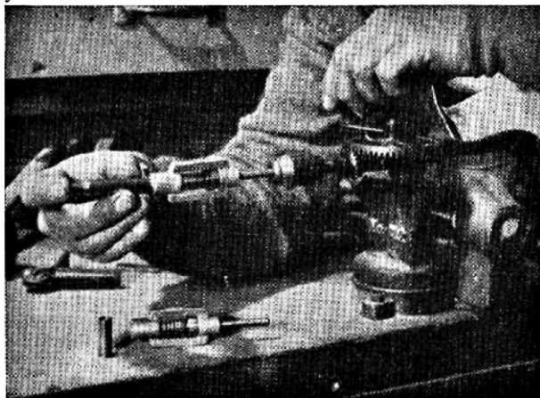
Wesnitzer primer pocket cleaner used in a chuck. Shell head fits into socket of cage for quick cleaning. Note cleaner on bench with .38 Special shell
