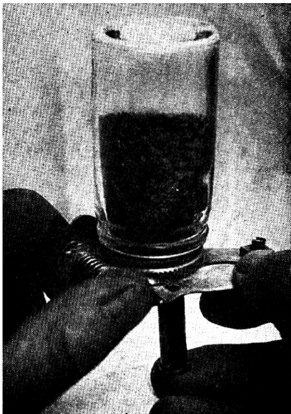
Homemade powder measures designed by A. J. Weinig. Golden, Colorado. Small mayonnaise jars are altered to drop proper charges directly into shell
