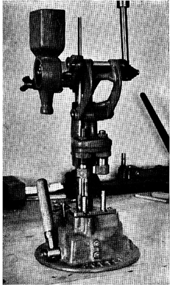
The new Potter Complete Loading Tool. The powder measure is mounted at the top of the machine and is optional with the purchaser. Sizing head holds both bullet seating die and resizing-de-capping unit. Operating lever with powerful toggle forces large sliding head containing dies down over shell. Auxiliary lever on the left side of the machine shows the primer seating device. Primer magazine may be seen sticking up between operating handle and powder magazine. Capacity 100 primers
