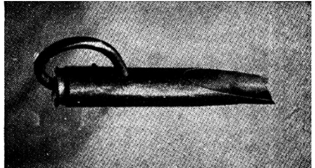
An excellent little scoop for running powder into the pans of your balance. This scoop was made from a new .30/06 shell. New cases work better for this, since the interior is clean and bright. The handle is a short brass rod which also serves as a plug in the primer flash hole
