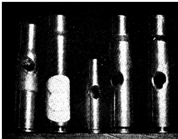
Cartridge cases used to record pressure. Left: 30/30 Winchester. This was previously drilled and the opening covered with a paper sticker to prevent spillage of powder. Beside it is a German Mauser cartridge manufactured by F.N. in Belgium. A sticker is pasted over it to hold the powder charge before the cartridge is inserted in the gun. This is the conventional foreign pressure cartridge. Center: .22 Hornet. Right: two 7-mm. cartridge cases used to register pressures. Mutilation around the hole is caused by pushing the gas check into the cartridge case in extracting from the gun
