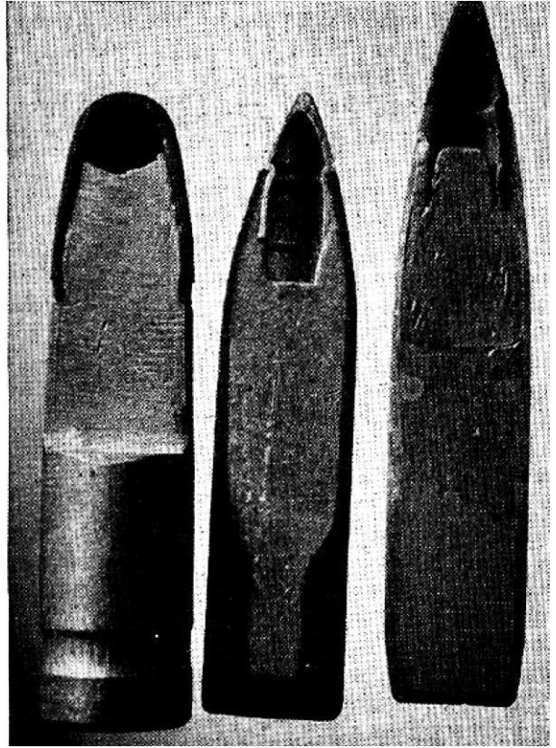
Types of foreign metal-case bullets. Left: The original Wesley-Richards .303 Magnum capped bullet. Center: The German (DWM) "strong jacket" bullet, heavy gilding-metal jacket designed so that the base portion will remain as a solid slug if the nose portion should completely shatter. This has the typical hollow copper-tube type of protected-point nose construction. Right: Another interesting German bullet, the RWS "H" jacket. Note how bullet jacket is folded in the center as a reinforcement. Also notice hollow copper tube and two-piece core.
