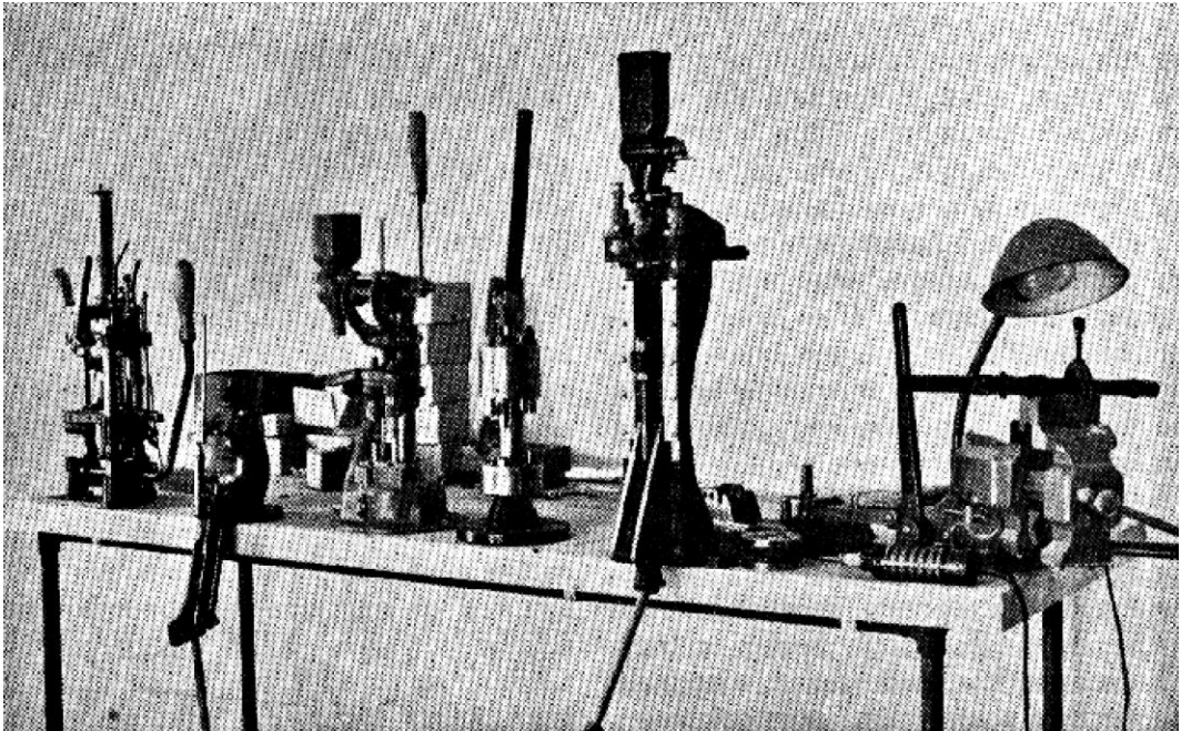
A good loading bench is extremely useful. The above bench in the author's laboratory was made of 0.75-inch iron pipe with a 2-inch birch top. The various tools may be used in any position, as they are attached to the bench with carriage bolts and wing nuts. The 12-gauge boxes in background are extremely useful to hold various change-over dies
