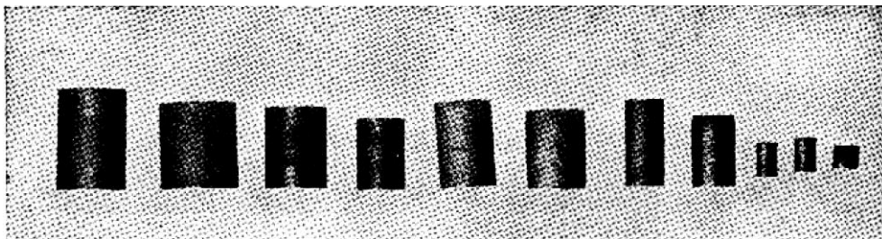
Pressure cylinders of various types designed for rifle, revolver, and cannon pressure tests. Left to right: Perforated French cylinder for taking light cannon pressure; French pressure cylinder for heavy rifle pressure; same for medium rifle pressure; same for light rifle; lead pressure cylinder used for revolver and shotgun pressure; same type of cylinder after compressing in pressure gun registering about 16,000 pounds; the standard copper crusher cylinder used for rifle pressure; same cylinder after compression in pressure gun registering 51,000 pounds. The tiny pressure cylinder on the right is a before-and-after version of the standard Frankford Arsenal copper crusher cylinder used for revolver pressures and one after compression at a pressure registering 21,000 pounds. Illustrations approximately actual size.
