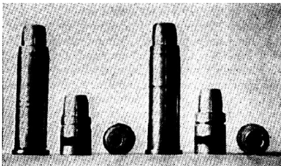
Heavy handloads for the .38 Special. Left: the Sharpe hollow-point bullet. Note small diameter of cavity. This is a straight cavity 0.1 inch in diameter. Right: the Keith bullet. This has a semi-conical cavity
