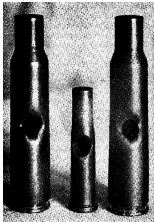
Cases as they are removed from a pressure gun: 7 mm. rifle and .22 Hornet. These were not drilled before taking the pressure
