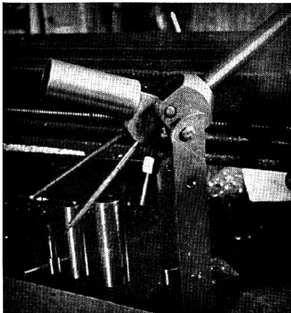
The present Sweany tool made for J. Bushnell Smith. This is Sweany's "commercial" model
