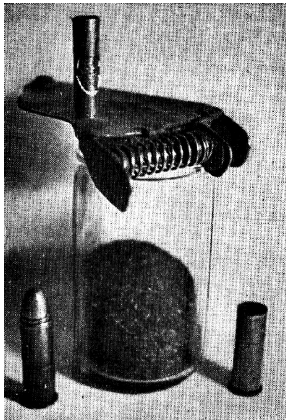
Close-up view of Weinig unit for measuring charges. Note adjustable metering tube
