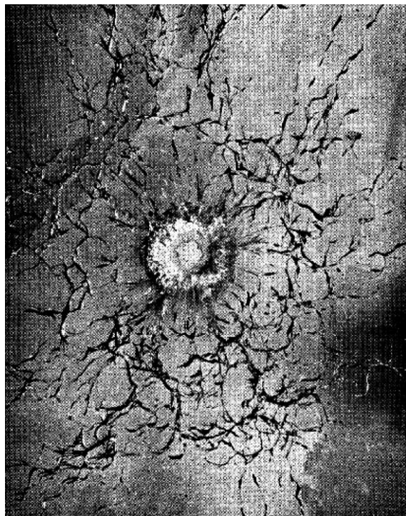
Shatter-proof windshield glass is excellent for comparing shocking power of different bullets. Windshield glass and windshield wings in sections large enough for test purposes can easily be obtained from auto dealers for the asking. The above section was shot with a .220 Swift soft-point bullet at a muzzle velocity of 4,200 f.s.
