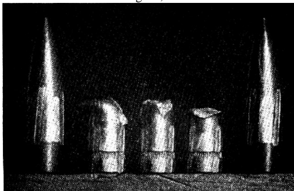
Effect on the bullet of shooting a tin-containing powder such as IMR #15½. These jackets are of gilding metal. Notice bright tin plating on the jacket where it contacted the bore, and absence of plating on the base section of boat-tail.
