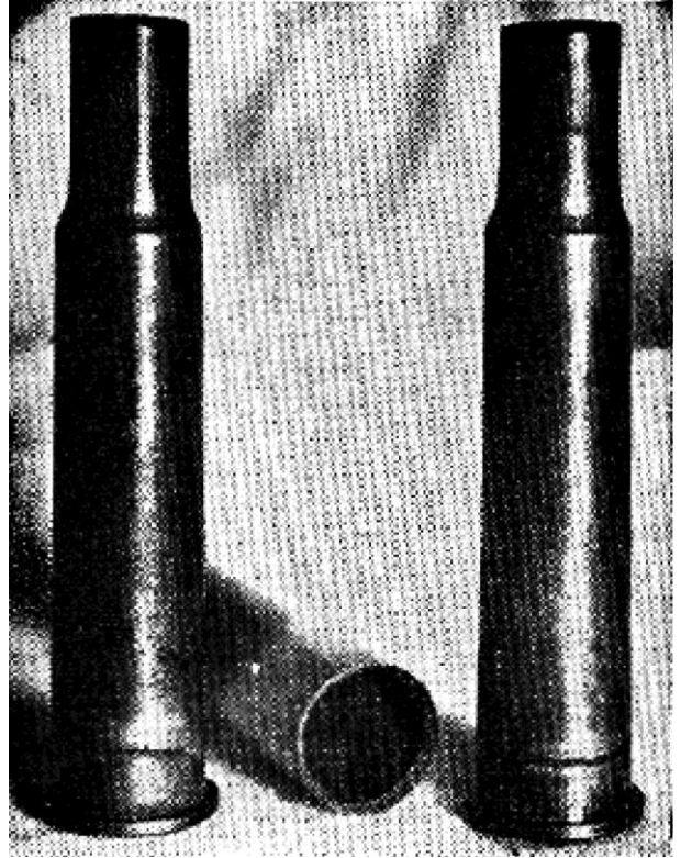
Poor brass and wartime cartridge cases. The 1918 Krag cases were made by Remington. These are frequently found and should not be used if they show the slightest sign of a rupture. Left and right, a partial rupture. Center, complete head separation. Had it not been for shooting glasses, the man behind that gun would have lost his eyesight
