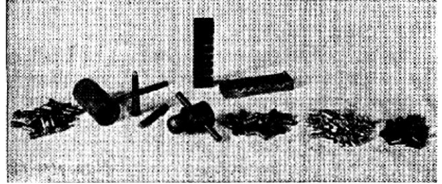
Home equipment for the manufacture of Hornet bullets from .22 short fired cartridge cases. This bullet swage was manufactured some years ago but did not prove successful, as it is extremely slow in operation, and Hornet bullets can be purchased much more cheaply than they can be manufactured. The cores are cast in the special mould as illustrated, and are inserted in the fired cartridge cases after the rim has been removed by forcing through a die. The bullets shoot well but are by no means perfect, as the various wrinkles cannot be removed even with extreme pressure
