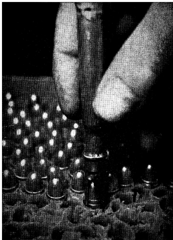
Removing lubricated bullet from a grease cake with a homemade cake cutter designed by A. J. Weinig of Golden, Colorado. Cutter is made from a .38 Special shell soldered to a .30/06 shell, the latter serving as the handle. Through the flash holes of both shells runs a wire to which is soldered a lip seen projecting over the top of the bullet. The side of the .38 Special case is cut out in part, and pressing on this plunger ejects the lubricated bullet from the cutter
