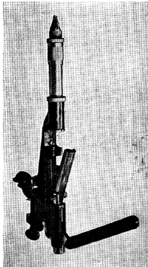
The old Bond Loading Tool. Capable of good work, but extremely slow in operation
