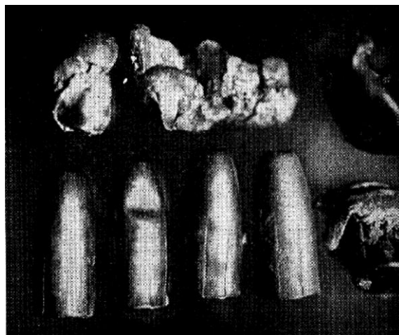
Hornet bullets may be tested for expansion by shooting into ordinary turf near small stakes pushed into the ground at ranges of from 100 to 200 yards. The above bullets were recovered at 100 yards and clearly show that hollow points do not expand. Note constriction of bullet where core flows forward within the jacket. The upset bullets were recovered specimens of the soft-point variety. Note the difference
