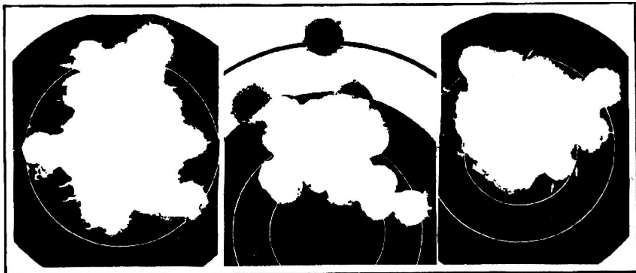
Three 100-shot targets. Machine rest twenty yards with handloaded .357 Magnum revolver ammunition. Loaded by the author. Fired at Smith St Wesson factory. Note: This ammunition was loaded for leading tests by the author and consists of measured powder charges—not precision-weighted charges. Left and center targets shot with standard Winchester bullets, standard factory velocity. Left target with grease wads, center target with colloidal graphite lubrication applied to bullet groove. Right target with 146-grain Sharpe Hollow-Point bullet. Colloidal Graphite Lubricant plus grease wad. Muzzle velocity 1,600 f.s. Each group was fired in a different barrel
