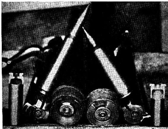
Breaching systems greatly affect the headspace of the gun. On the left is a standard Springfield barrel with a cartridge inserted. Note extractor groove in the large portion of the cartridge case sticking out of the chamber, due to the shape of the breach of the bolt. The entire extractor groove is visible. Right: A close breaching system designed by J. B. Sweany of Winters, California, for the Springfield action. Note alteration of bolt and way cartridge case drops into the chamber so it seats flush with the mouth of the barrel. The barrel is turned out square rather than coned as in the Springfield standard system. This gives complete support to the weak portion of a cartridge case and prevents stretching
