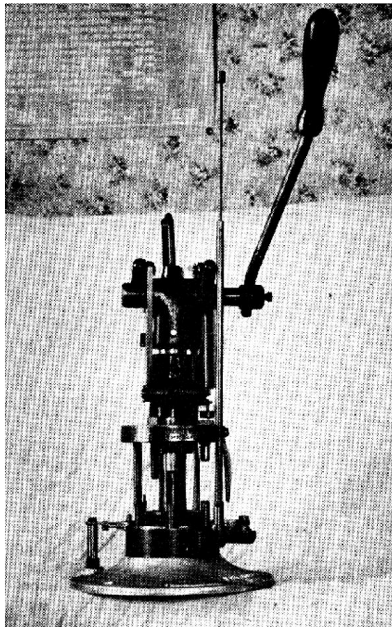
The most expensive model of Star Loading Machine. This is superior to all other loading machines in its speed and uniformity of operation. One merely feeds shells into the rotating turntable and bullets into the bullet-seating station, operating the lever each time. The fully loaded cartridge is automatically discharged through a discharge slot at each operation of the handle
