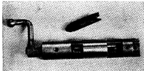
Wilson's latest adjustable trimmer, in which one unit, equipped with proper shell holders, will handle all cases from the .22 Hornet to the .375 H. & H. Magnum. This trimmer, because of the adjustable feature handling all calibers, does not chamfer the inside of the case neck and turns up a very slight burr both inside and out. The auxiliary burr-removing tool is supplied with this and is capable of handling all calibers. It is very simple to use
