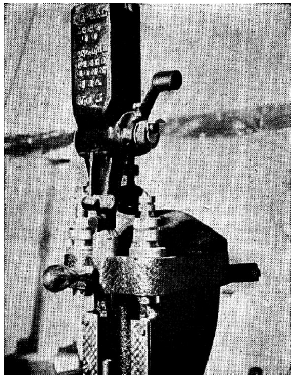
The Rotating Turret of the Universal Tool with Ideal powder measure properly mounted. One merely swings the rotating turret head from side to side to line up the various units for resizing and de-capping, throwing powder charges, and bullet seating
