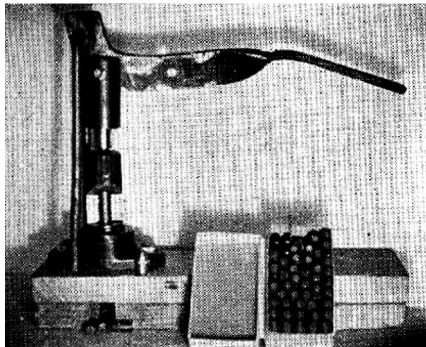
Homemade bullet swaging or resizing tool made by A. J. Weinig of Golden, Colorado, in part from the Belding & Mull bullet resizer. The side is cut from the die to permit easy insertion of bullets. This tool will resize metal-cased bullets readily
