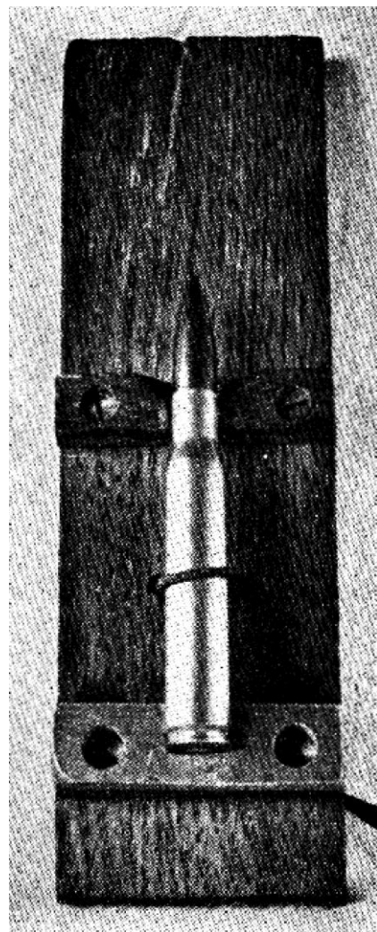
A homemade bullet spinner designed for checking concentricity of loaded cartridges. The device is clamped in a vise of some sort and the cartridge case laid into the proper groove. The neck operates in a V groove. The cartridge case is spun by pulling back and forth on the string wrapped around it. Wobble of the bullet is noted during the inspection
