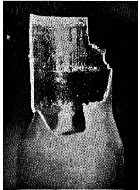
Effect of mercury on a cartridge case. Brass became extremely brittle and the loaded cartridge was broken by pressing on the bullet
