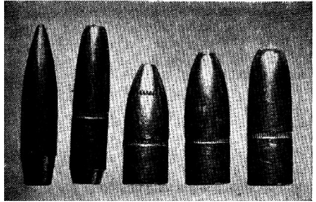
Winchester and Western Magnum bullets are excellent to behold. These five bullets represent the latest additions to the H. & H. Magnum series. Left to right; the 300 Magnum 180-grain Boat-Tail Match (note absence of cannelure); the 220-grain Boat-Tail short exposed soft-point; the three bullets available for the .375 Magnum in standard loadings—235, 270, and 300-grain. The lighter weight is a hollow-point, the others soft-point.
