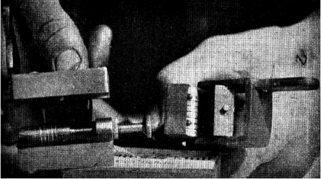
Two interesting bullet moulds. Left: The old obsolete Ideal for casting different lengths and weights of rifle bullets in a given caliber. Length of bullet was determined by adjusting the screw and sliding cavity plug. Right: An old H. M. Pope mould with peculiar double cut-off plates. Bullets were poured from the point. This was supposed to cast more perfect-base bullets
