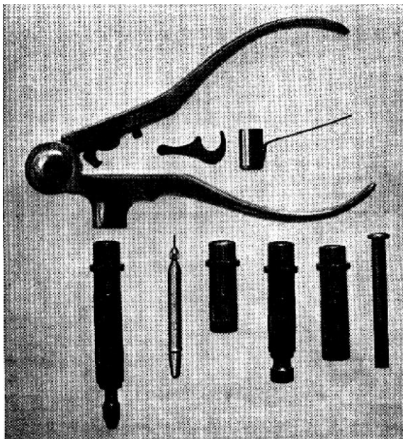
Ideal tong-type tool designed for military rifle cartridges of the rimless type. Adjustable chambers
