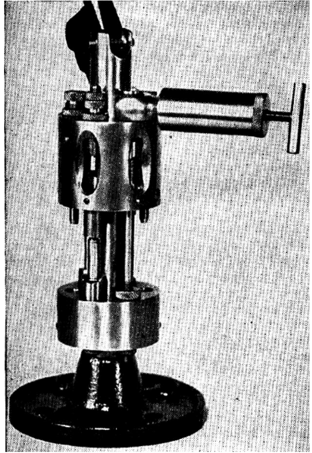
Lubricating attachment for Jordan Loading Tool (see Chapter XXII)
