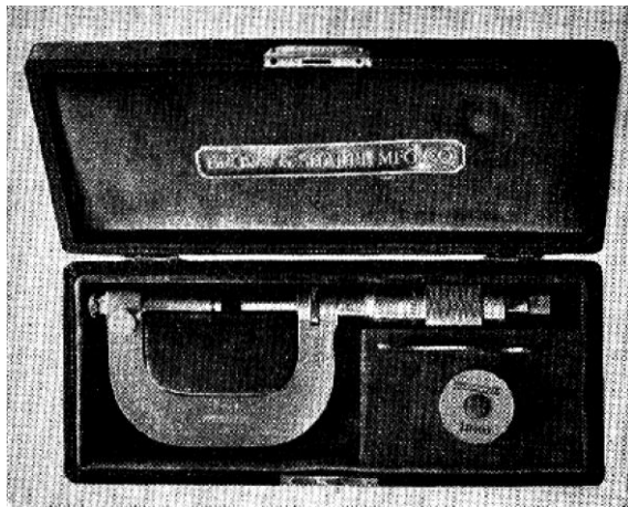
Brown & Sharpe 2-inch Micrometer with Adjustable Anvil. This is an extremely practical tool and serves the purpose of two separate instruments. It has a capacity ranging from zero to one inch, as illustrated above, and when the anvil is slid back to proper position, the capacity is increased from one inch to two inches. A standard which is sent with the instrument is used to check the adjustment
