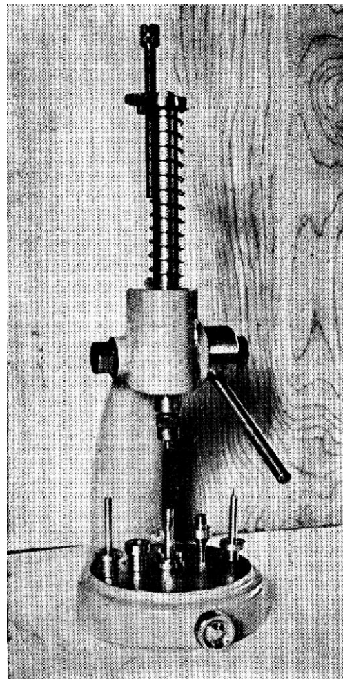
Special homemade straight-line tool designed and manufactured by H. A. Donaldson, Little Falls, New
