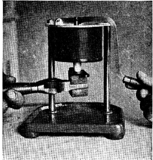
The latest thing in a melting pot for bullet casting. The new Potter double-standard type, electric-power cord plugs into rear of melting pot. Standard electric-iron plug is used
