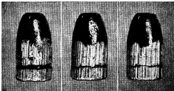
Leading can seriously injure the accuracy of any gun. The above recovered revolver bullets were shot from a badly leaded bore
