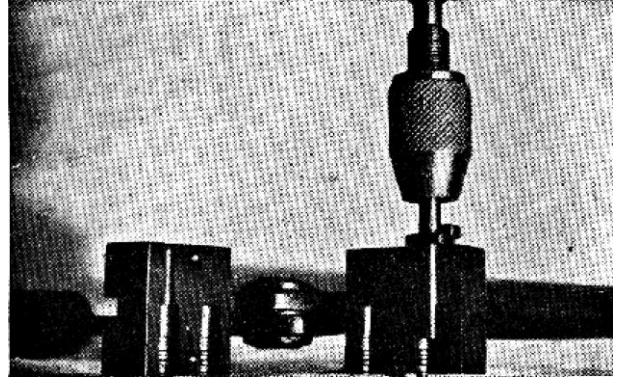
The Hensley mould with hollow-point attachment
