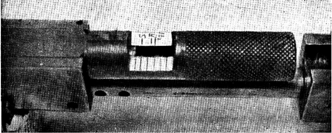
Homemade alterations of Belding & Mull bullet-seating die by A. J. Weinig, Golden, Colorado. A section is cut from the seating chamber, barely exposing the case neck and bullet base. Care must be taken not to remove too much metal. Lines are filed on the flat surface to act as gauges and check the adjustment visually. This also permits air to escape from the seating chamber and prevents the accumulation of grease, which frequently changes seating depth. An excellent idea
