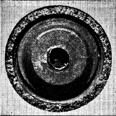
Microphoto by E. M. Chamot Hornet cartridge case which had been primed with a mercuric primer of the non-corrosive type (new case) and fired once. Head pulled off in resizing die. Note crystalline structure of the break around the edge. This is an excellent example of what mercury does to brass
