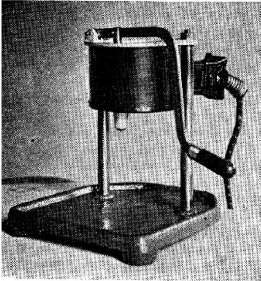
The latest thing in a melting pot for bullet casting. The new Potter double-standard type, electric-power cord plugs into rear of melting pot. Standard electric-iron plug is used
