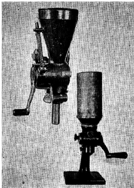
Top: The Comer measure. An excellent and extremely uniform type. This is about as fast as any measure the author has ever tried. Bottom: The old Frankford Arsenal powder measure with the funnel hopper removed and a straight cylinder hopper used in its place
