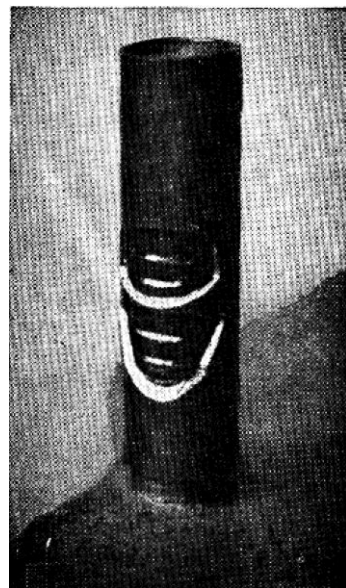
Close-up of metering tube on homemade Weinig powder measures. Note scale lines filed into tube to permit adjustment for different weight charges
