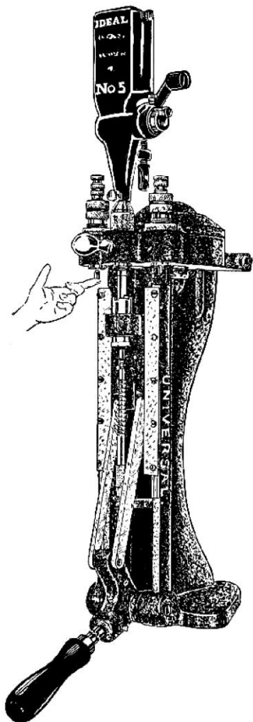
U. S. Patent No. 2004420 The Universal Tool complete. At all times it is set up for the various stages of a given caliber
