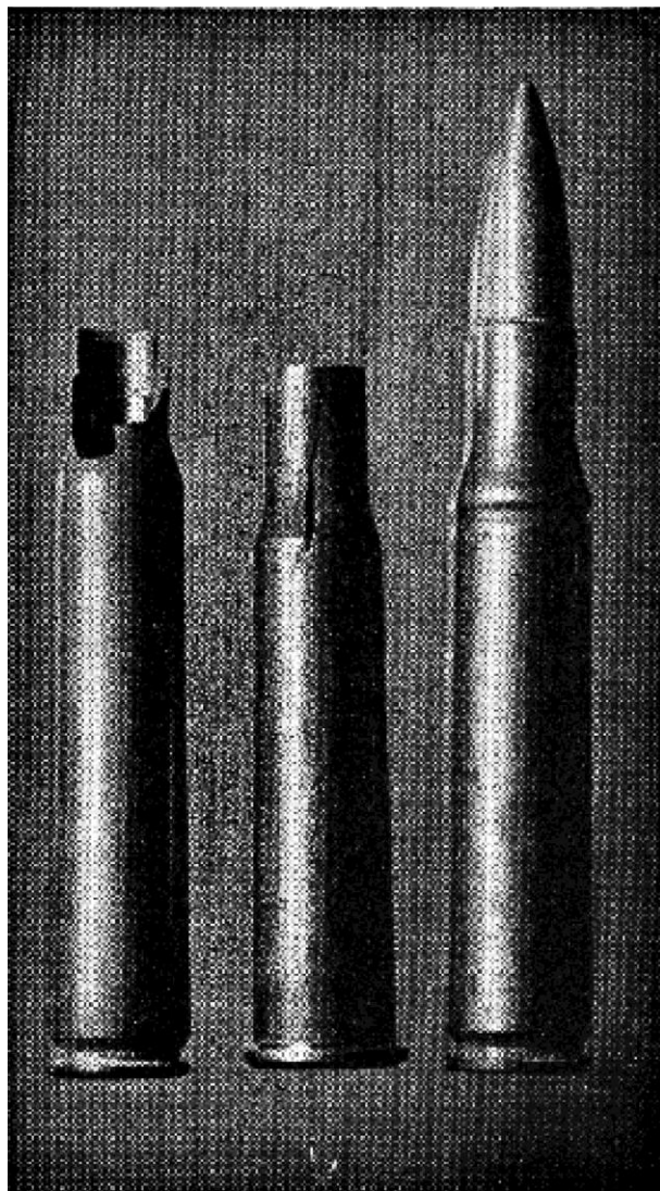
Mercuric primers have a bad effect on cartridge-case brass. Left, three mercuric primers used in the Springfield case. Final loading was broken in the fingers after the bullet was seated. Center, Krag cartridge fired once with a mercuric primer. Right, the primer is stronger than many people think. This wartime cartridge was shot on a target range. It appeared to misfire. Examination showed that the flash hole had not been punched and the force of the primer drove the cartridge into the chamber, buckling the shell at the neck
