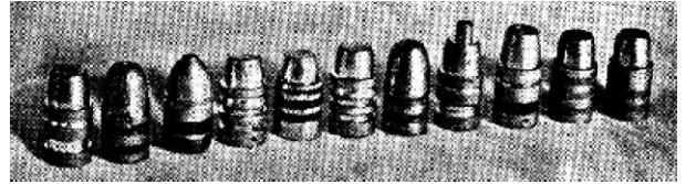
A few revolver bullets for the .38 Special showing the variations possible in different styles and weights for different purposes
