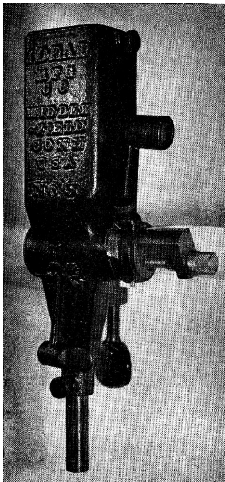
Latest version of Ideal powder measure—the No. 5 Micrometer. This measure does not prove to be as uniform on light revolver charges as on heavy rifle charges, owing to the micrometer arrangement
