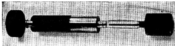
An excellent hand bullet seater of Belding & Mull manufacture designed for use with the Model #26 tool. Various of these units are used by the author in seating special bullets, as it is capable of first-class work. It can be used to crimp or not, as desired, and is readily adjustable for seating depth. The cost of these tools is exceedingly low
