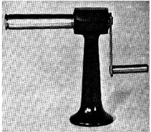
The Jordan case trimmer. The cartridge case is stopped in its socket by the shoulder. Brass is trimmed to proper neck length on turn of the handle
