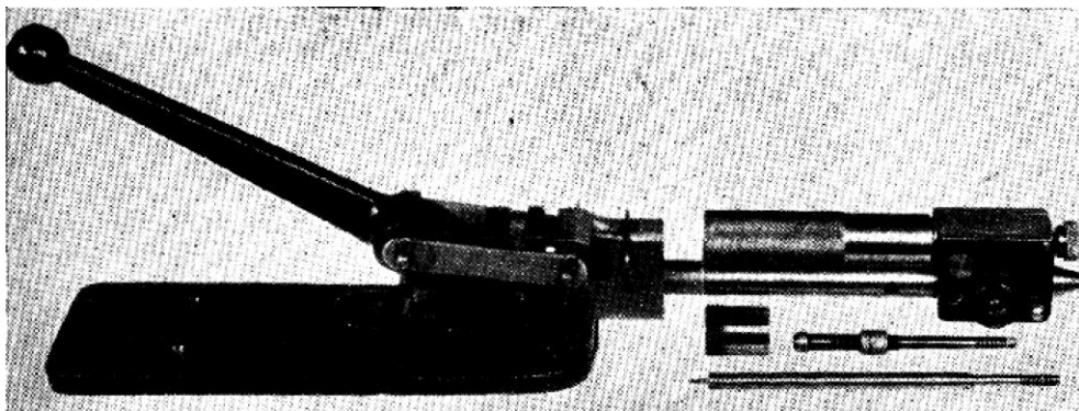
Belding & Mull Model #28 Loading Tool set up for bullet seating in the .30/06. Various accessories are shown for neck sizing, expanding, and de-capping
