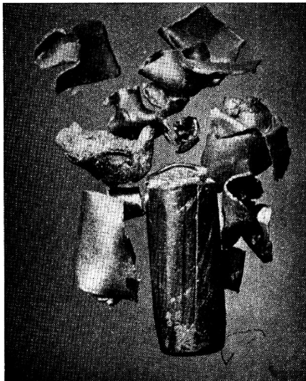
The RWS "H" jacket bullet after firing. Note complete shattering of nose portion and almost perfect remainder of the base section. An excellent hunting bullet.
