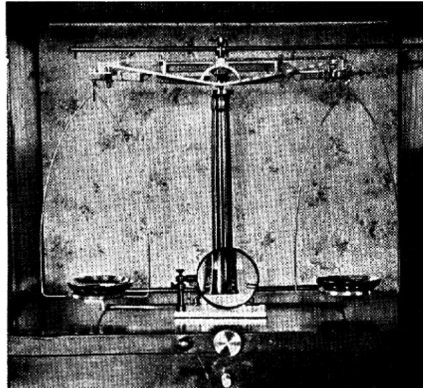
Close-up of Becker cabinet balance showing magnifier lens used to read the index scale.
