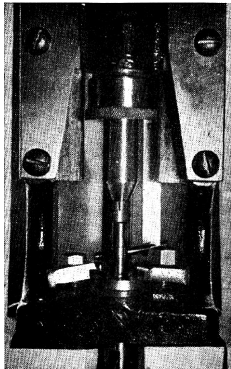
The Ideal Armory press set up to full-length resize cartridge cases and de-cap at the same time. Tool set up in .38 Special. Note shell holder clamped by means of special clamp nuts
