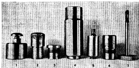
Straight-line bullet seater and shell re-sizer designed and manufactured by L. E. Wilson of Cashmere, Washington, for his own use. Units as marked are: (1) adjustable cap for bullet seating, (2) plunger for case neck resizing, (3) bullet seating die, (4) body of the tool with neck die in position, (5) sleeve for holding case in straight line within the tool, (6) die and reamer die for use in reaming case neck, (7) the case neck reamer. A punch for removing resized shells from the neck die is not illustrated. In use, the unit No. 5 is slid into the case neck body part No. 4. The plunger No. 2 is used to force the case and its sleeve to proper depth in the neck sizing die shown at the bottom of the body No. 4. If it is desired to ream case necks, the neck-sizing die is placed with No. 6, which is also a neck die but has an unusually long pilot to permit of reaming and trimming the cases while still clamped solidly in the die. An extreme precision tool
