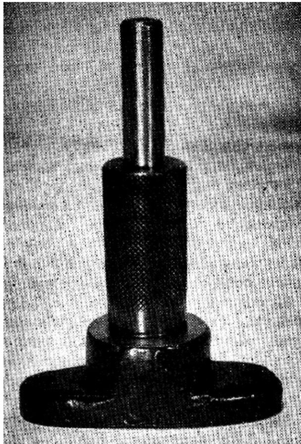
A very practical bullet sizer for the man who does not care for an expensive machine. The bullet is first lubricated by some process similar to dipping, dropped into the top of this sizer, and then shoved through with the plunger, base first
