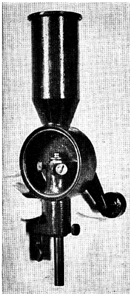
The Bond measure. Note revolving cylinder operated by crank. Metering chambers illustrated in the discharge position
