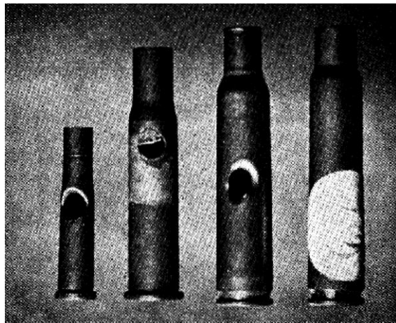
Cartridge cases which have been used in a pressure gun. Notice hole blown through brass case during the taking of pressure. Left to right: .22 Hornet; .30 WCF; 7-mm. Mauser. Right: an 8-mm. Mauser case prepared at the laboratory for the taking of pressures. Note large hole drilled in cartridge case and covered by a white paper sticker
