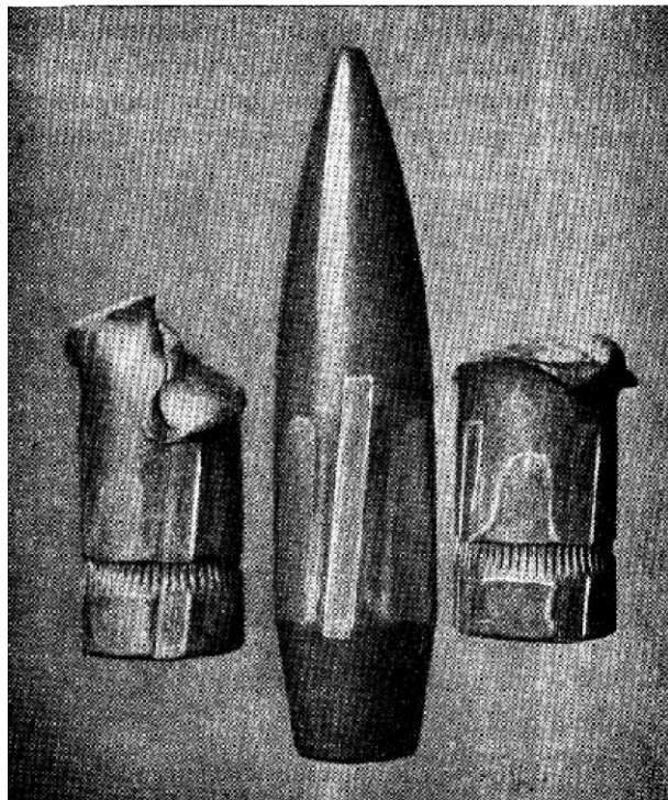
Tin-containing powders, such as the Du Pont IMR series ending in "1/2," foul barrels with metallic tin, plating the bullet where it contacts the bore. The above bullets, recovered from a sandbank, include: left, Remington 110-grain fired with charge of IMR #15½; center FA un-cannelured 173-grain boat-tail, fifth shot with a powder containing no tin after fouling barrel with ten of the previous loads; right, Remington 110-grain fired with a no-tin powder, tenth shot after one on extreme left. Note traces of tin plating even on this bullet where it contacted the barrel.
