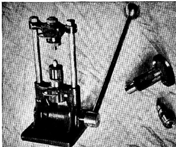
The new Bond Model "D" Loading Press, the best-designed press ever turned out of the Bond factory. It is quickly changed over for different stages of operation. Press as shown above is set up for bullet seating for the .38 Special, and delivers excellent work. Dies do not screw into the holders but slip in and are locked by means of the large horseshoe springs visible in the top and bottom center of the picture
