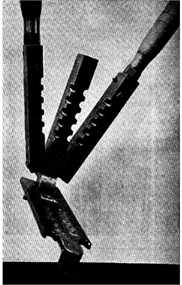
Another multiple mould by Fielding B. Hall. This casts ten .38 Special bullets at a time. Notice twin bullet moulds combined on one set of handles. Extra heavy sprue cutter on top readily shears sprue from ten bullets
