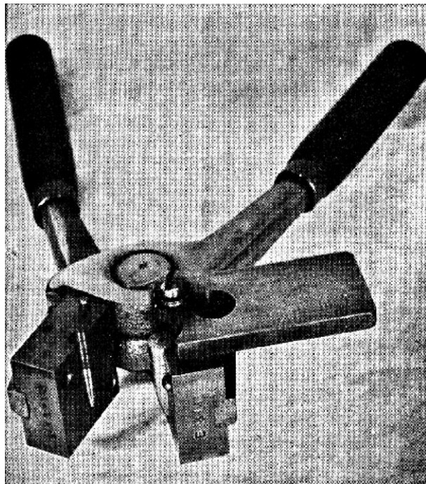
The Belding and Mull single-cavity mould for a pointed cast rifle bullet. Note large handles, sturdy construction of blocks, and large and easily handled cut-off lever
