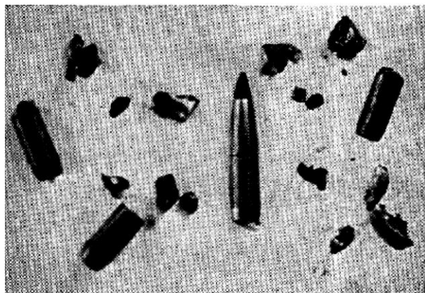
The RWS 7-mm. 173-grain "H" jacket bullet. Notice fold in bullet jacket and perfect condition of recovered bases. Fragments of the nose are also clearly visible.
