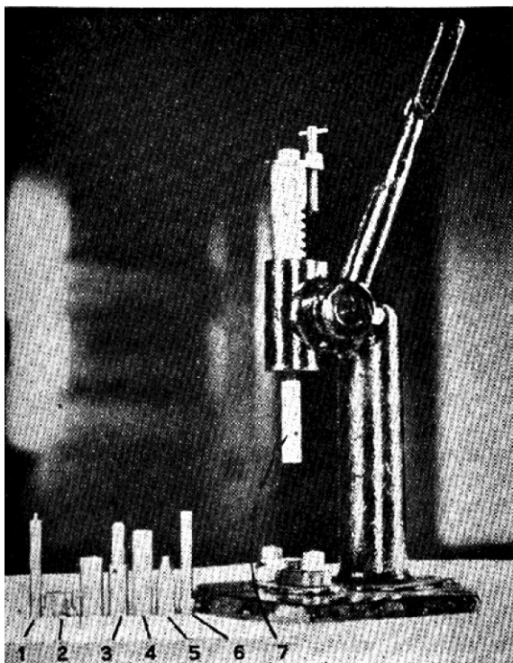
The Yankee Bench Loading Press, Model D. Various accessories are shown: (1) de-capping punch, (2) shell holder, (3) muzzle expander, (4) muzzle re-sizer, (5) primer seater, (6) priming stake and (7) bullet seater
