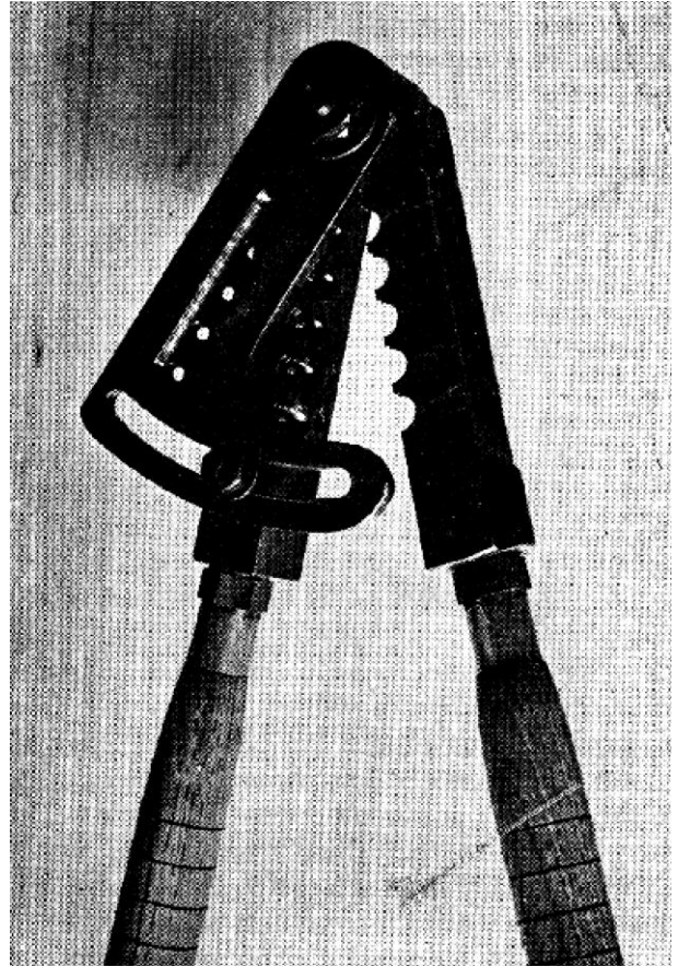
Gang moulds are often useful for speed casting. This one, designed by Fielding B. Hall of Los Angeles, throws five .38 Special bullets in a single cast
