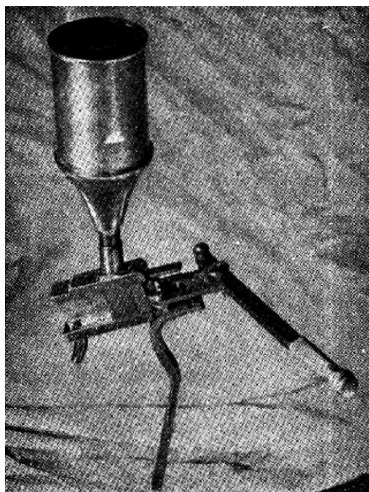
A homemade powder measure which works fairly well for throwing handgun charges. The upright portion is clamped in a vise or attached to the side of the loading bench in an upright position by means of screws. The measure was built from odds and ends by a dentist
