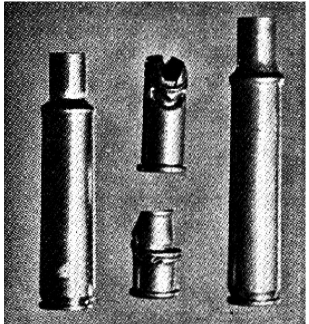
In sizing shells be sure you set your dies properly. The above cases were ruined through improper set-up
